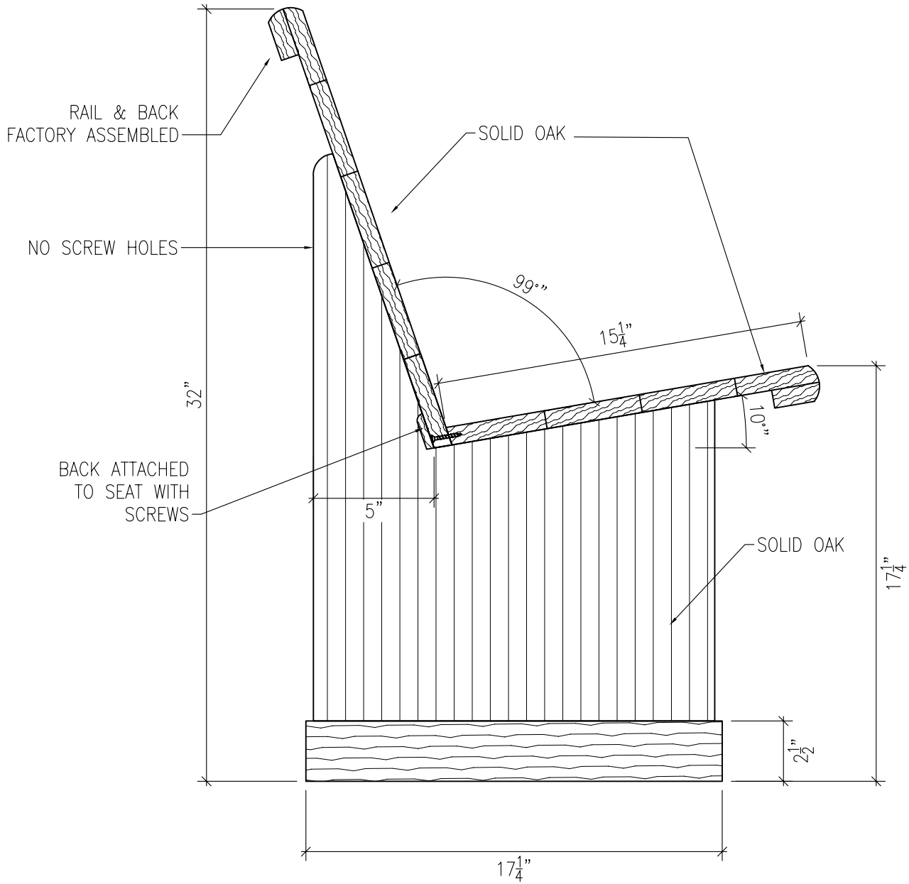
1 A VERTICAL SECTION MODEL "A" SCALE: 2" = 1'-0"
