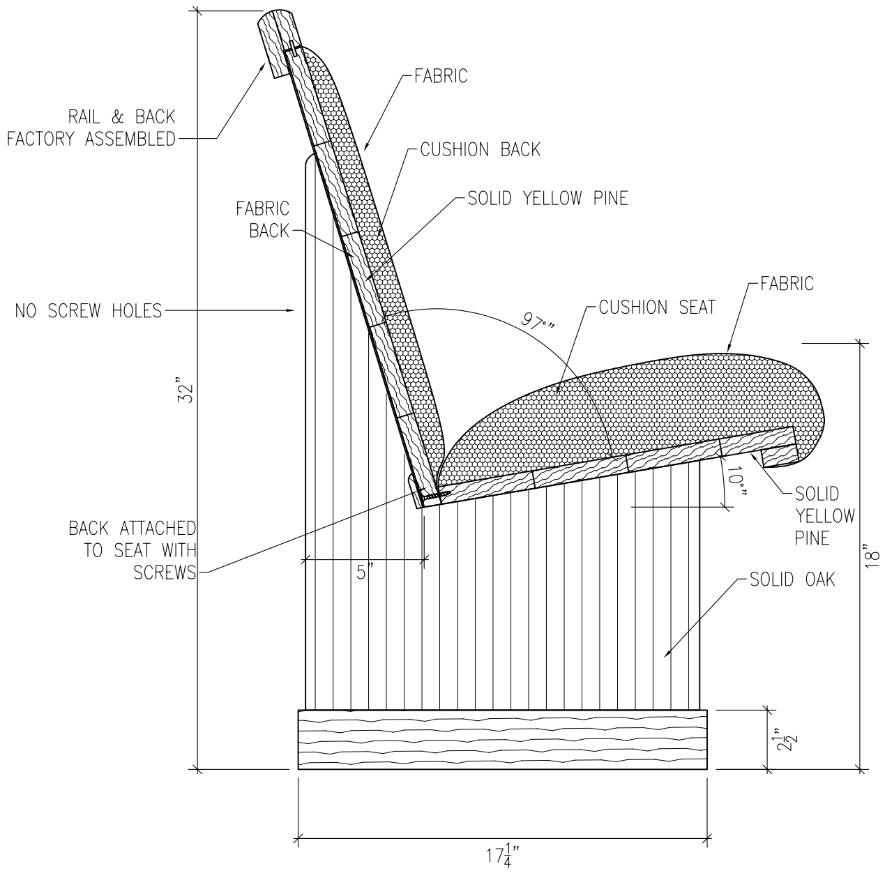
1 C VERTICAL SECTION MODEL "C" SCALE: 2" = 1'-0"
