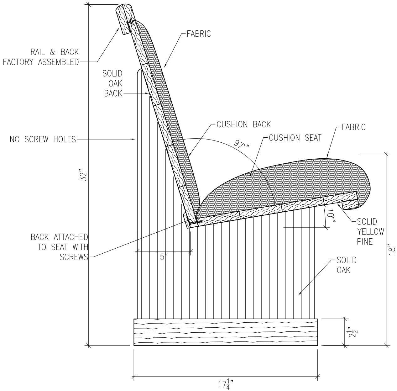
1 D VERTICAL SECTION MODEL "D" SCALE: 2" = 1'-0"
