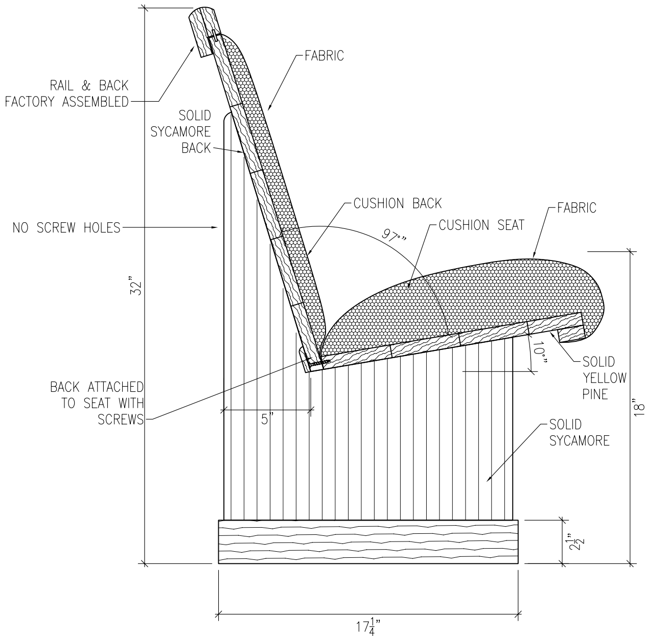
2 D VERTICAL SECTION MODEL "D" SCALE: 2" = 1'-0"
